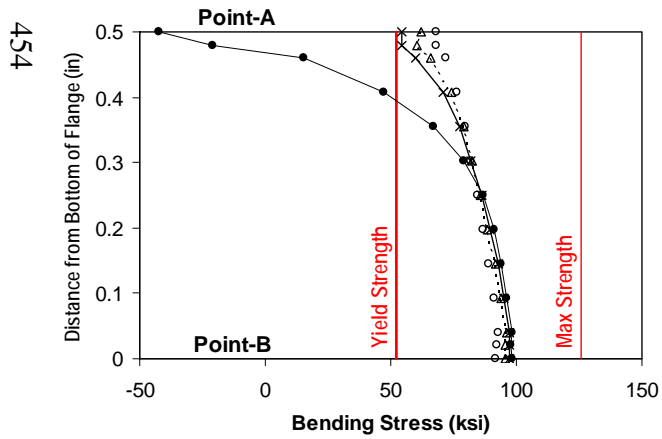
(b) Bending Stress along Thickness of Flange
