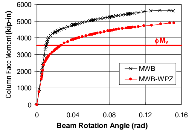
(h) Column Face Moment vs. Rotation Angle
