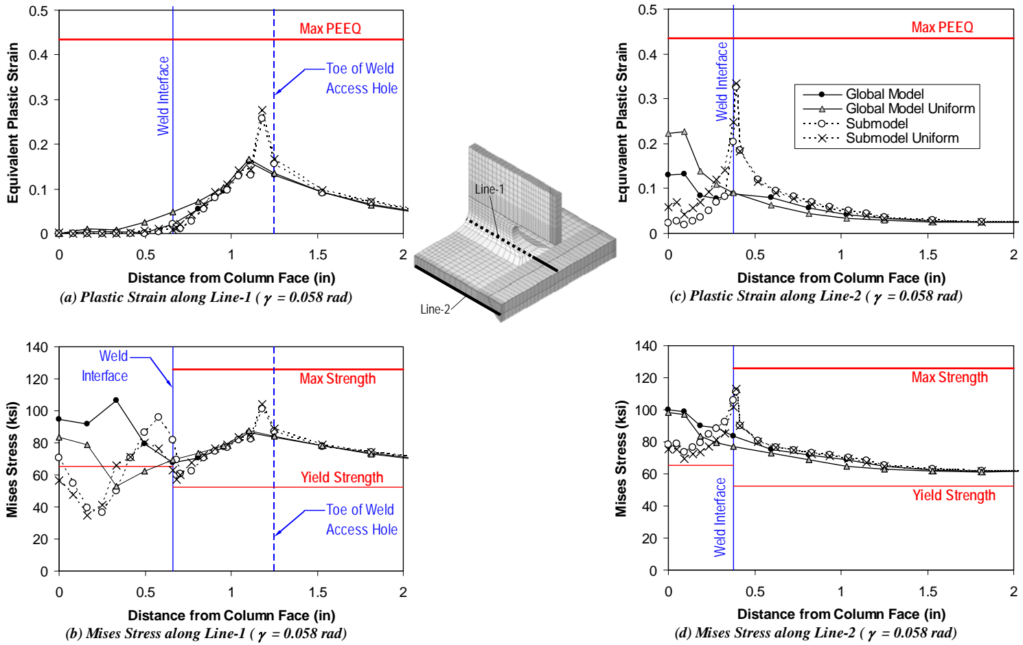
Figure 6.17 Comparison between global model and submodel
