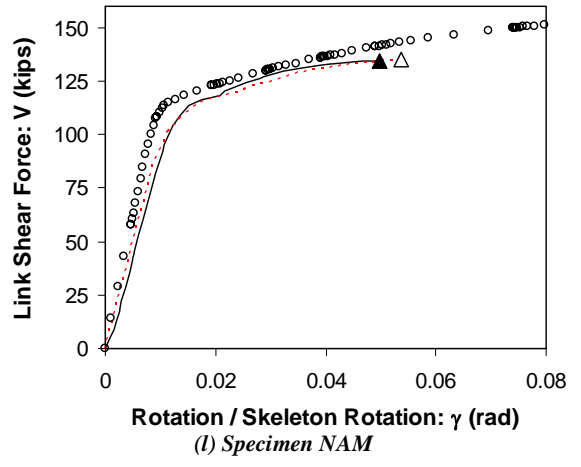
Figure 6.8 Simulated loading curve vs. skeleton curves (Continued)
