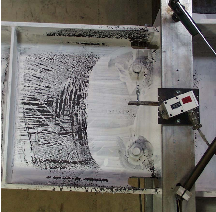
(a) Yielding around shear tab (0.03-2N)
