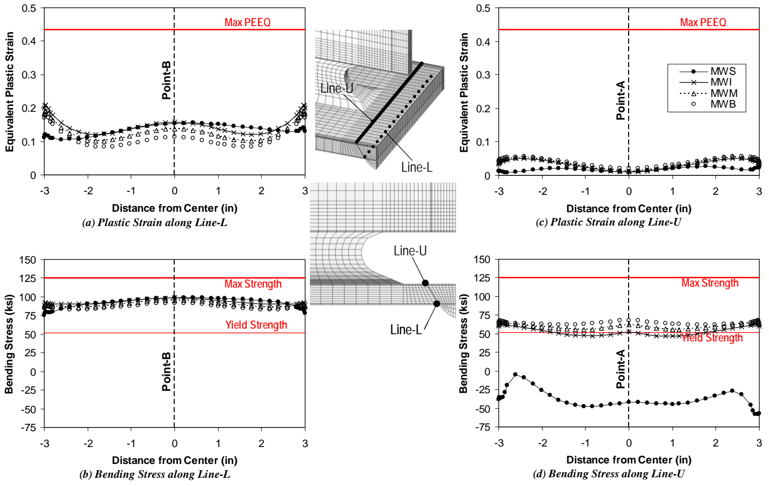
Figure 6.21 Effect of link length on the link flange-groove weld interface
