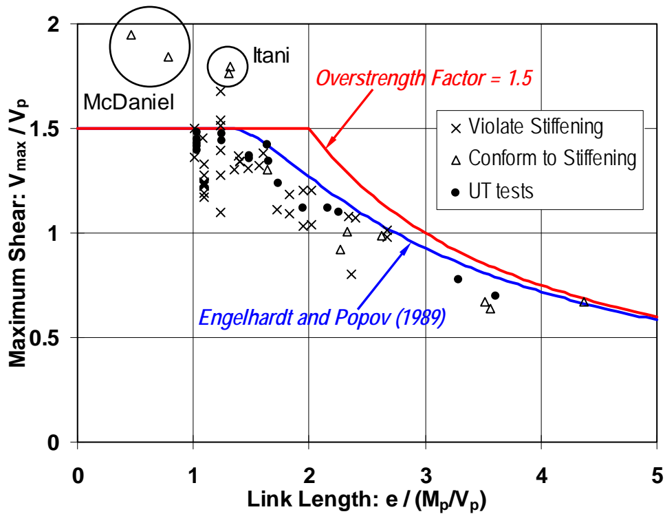
Figure 2.7 Link maximum shear strength
