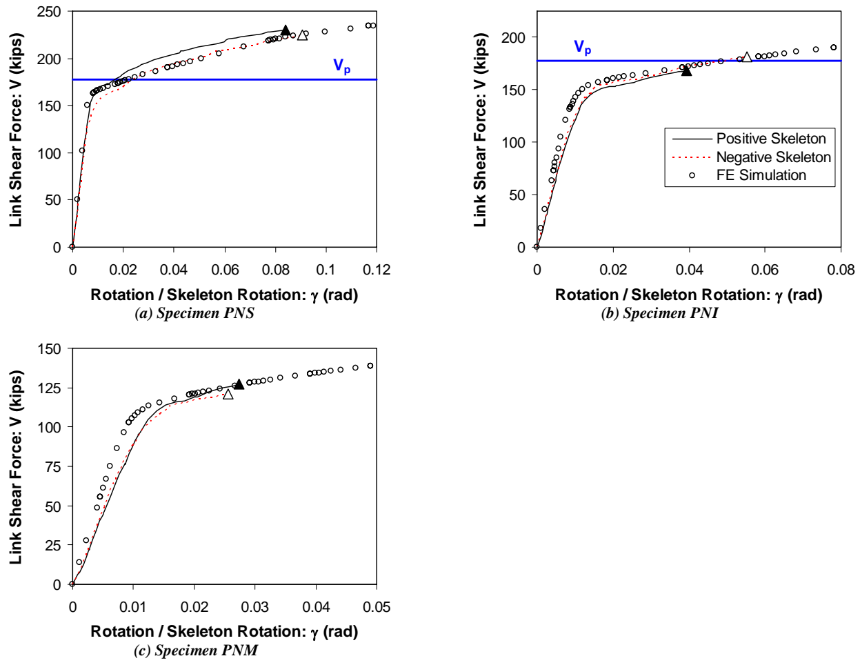
Figure 6.8 Simulated loading curve vs. skeleton curves
