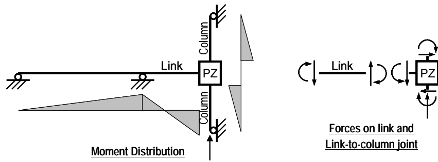
(a) Forces in link-column specimens
