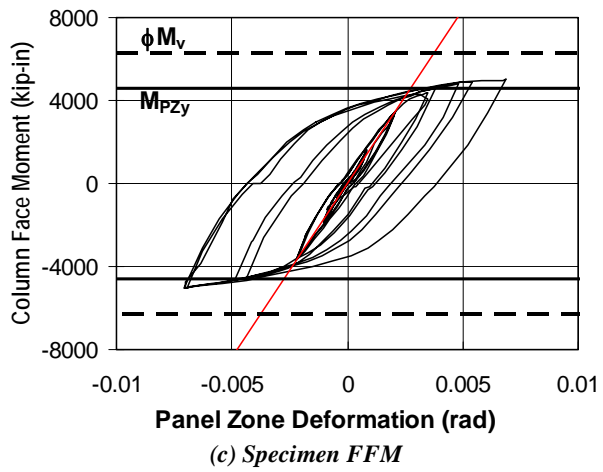
Figure 5.28 Panel zone deformation vs. column face moment
