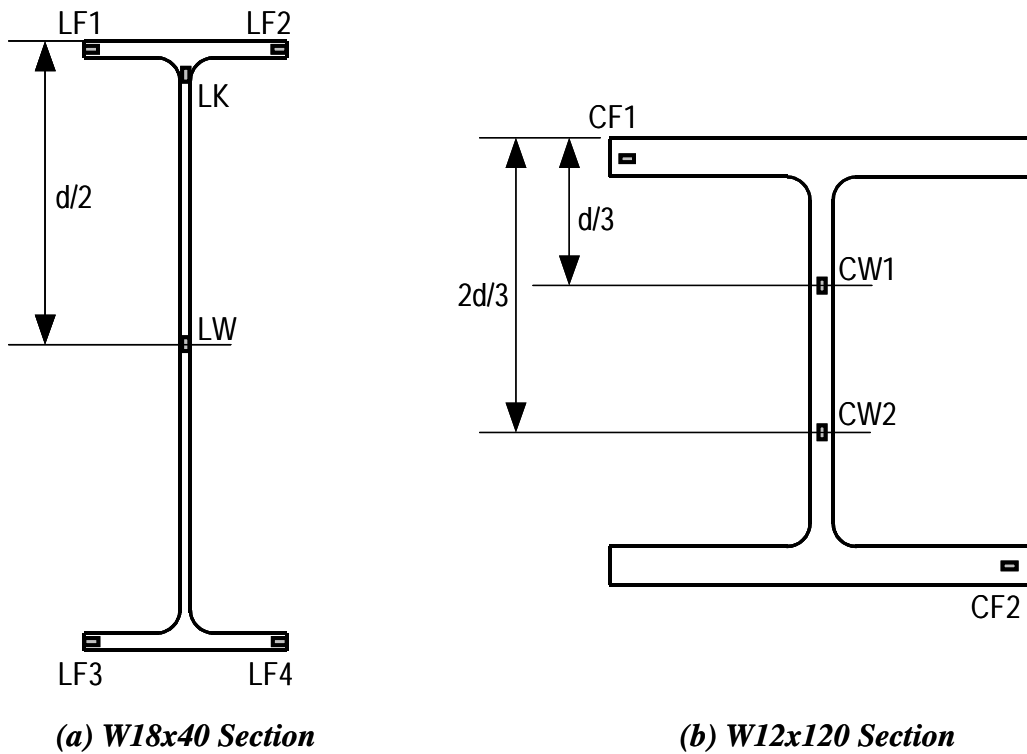
Figure 3.16 Tension coupon locations
