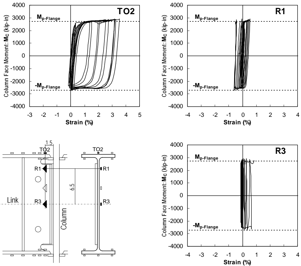
Figure 5.24 Longitudinal strain history in Specimens MWS
