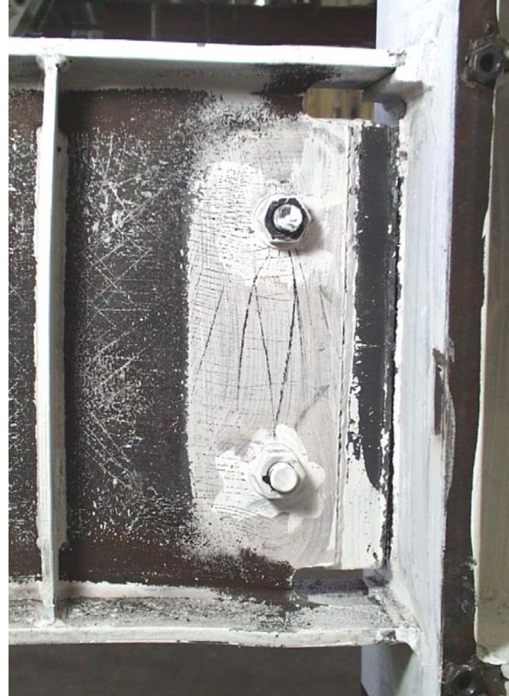
Figure 4.24 Photographs of Specimen FFS-RLP (Continued): (c) (Above) Fracture in bottom edge of shear tab weld (0.04-1N); and (d) (Right) Link-to-column connection after test
