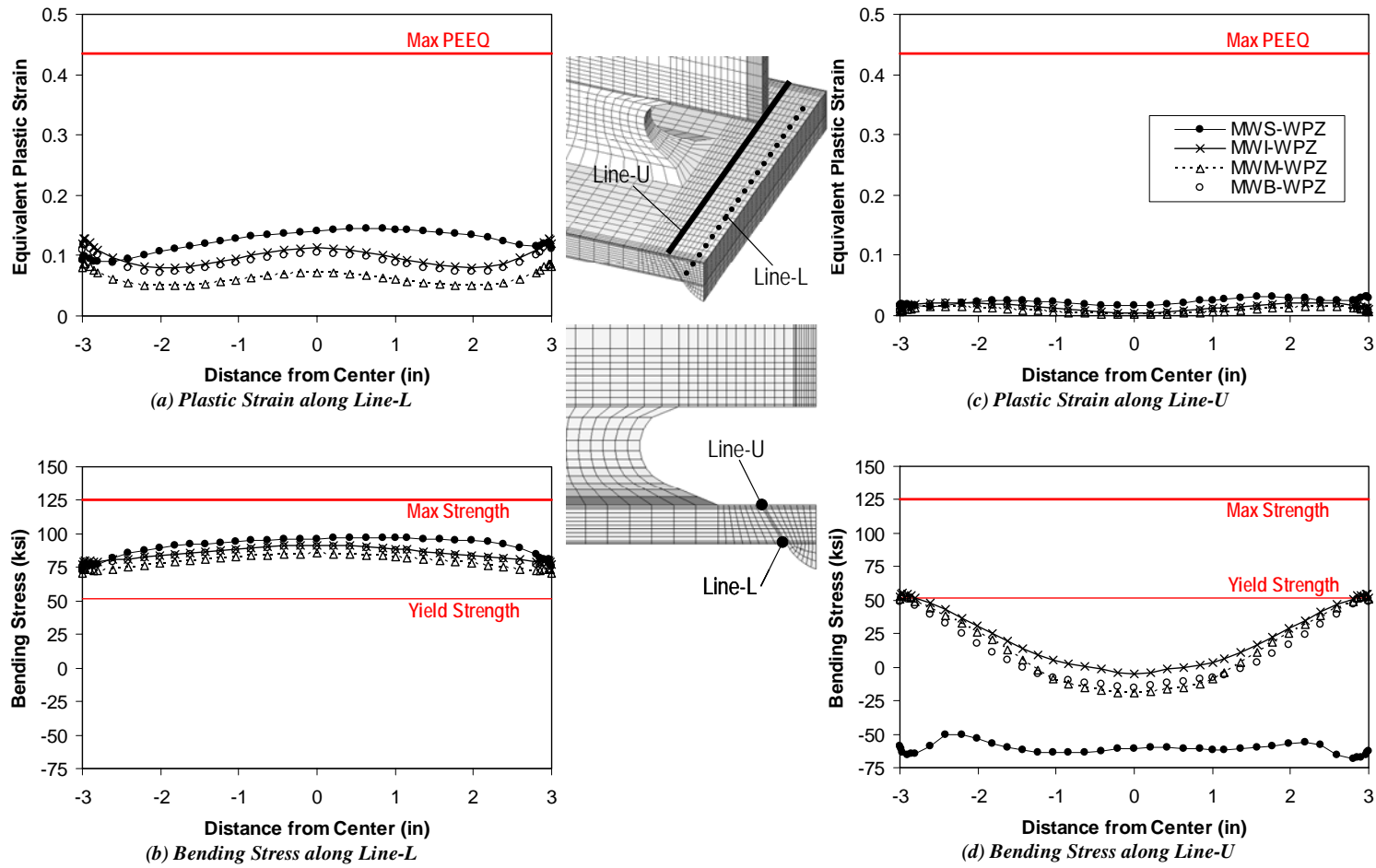
Figure 6.36 Effect of weak panel zone on link flange weld interface
