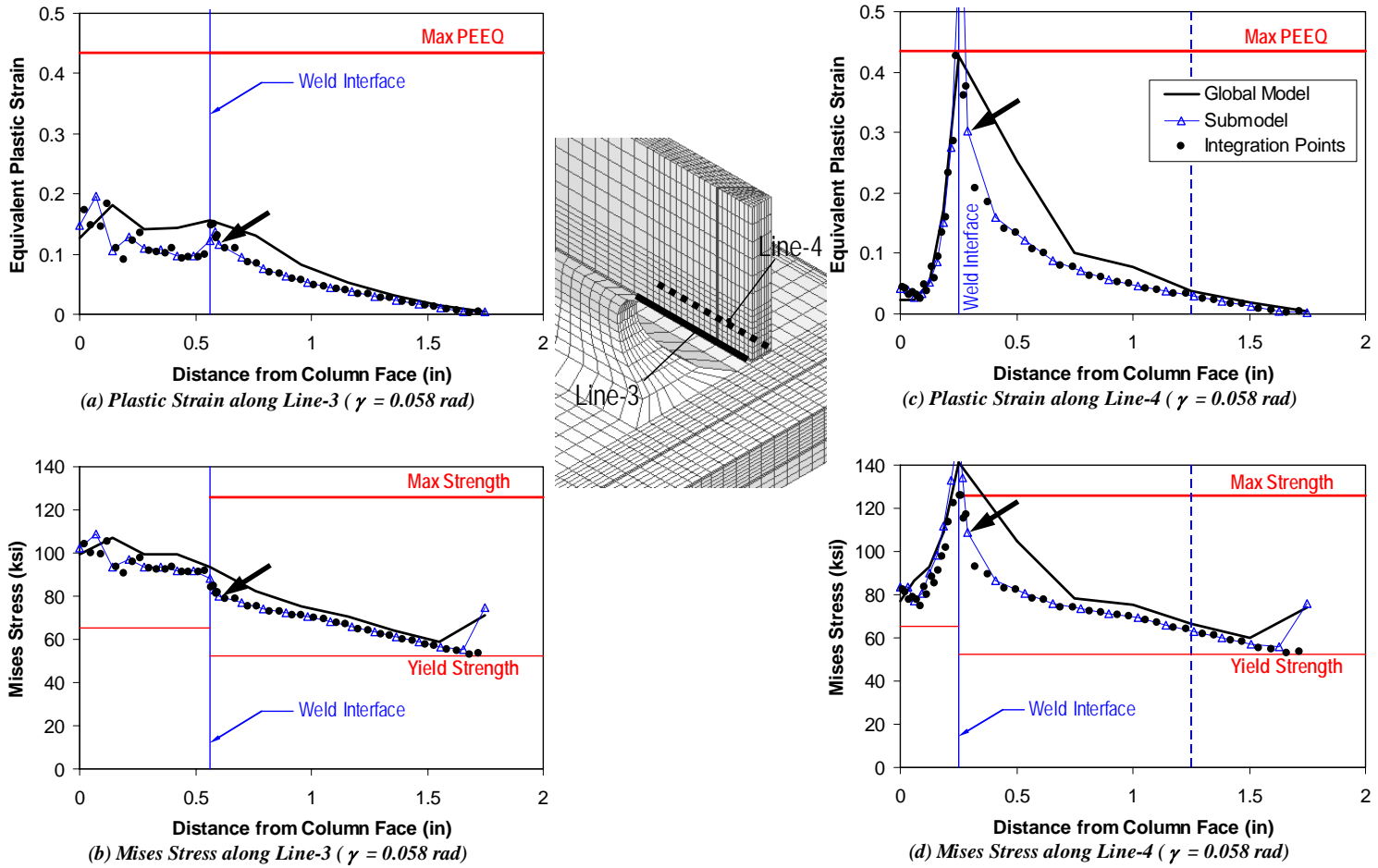
Figure 6.19 Sampling points near link web groove weld
