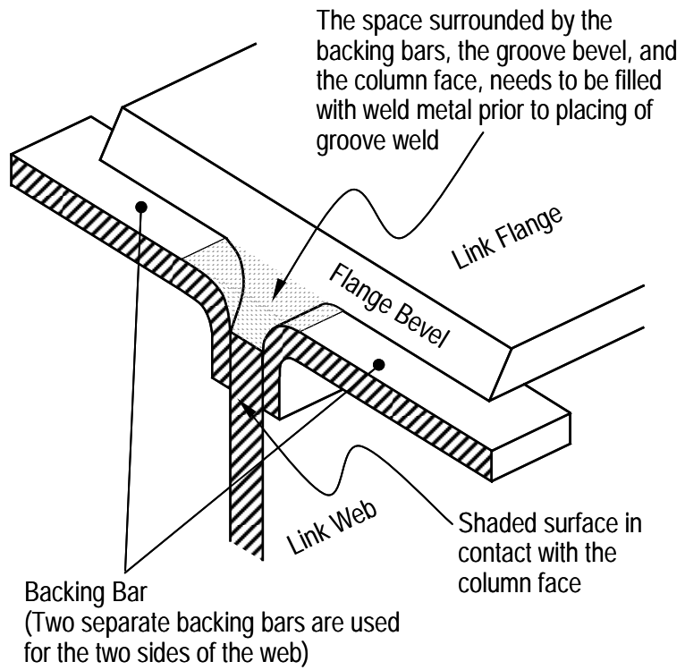
(a) Customized backing bar for NA-connections
