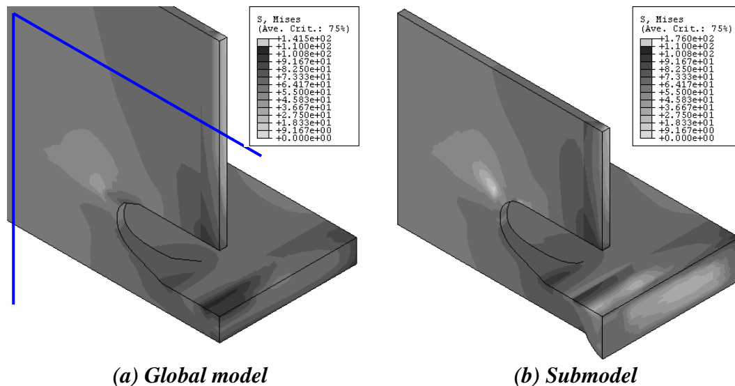
Figure 6.15 Mises stress distribution in global model and submodel
