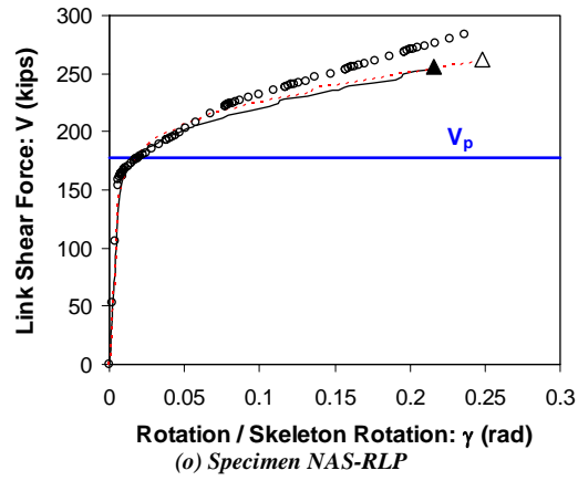
Figure 6.8 Simulated loading curve vs. skeleton curves (Continued)
