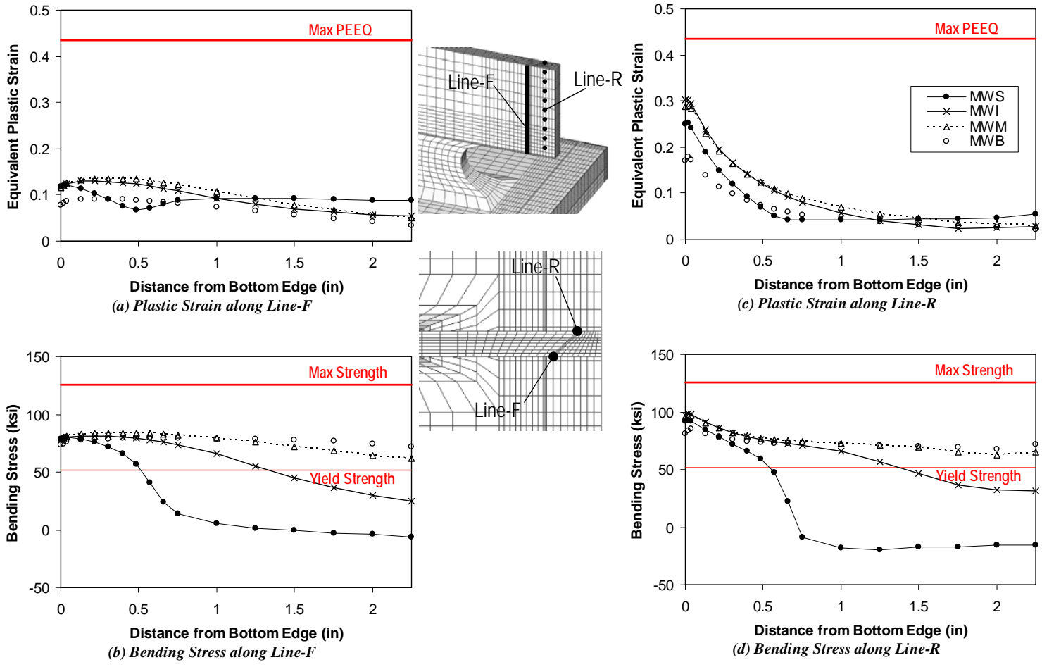
Figure 6.24 Effect of link length on the link web-groove weld interface
