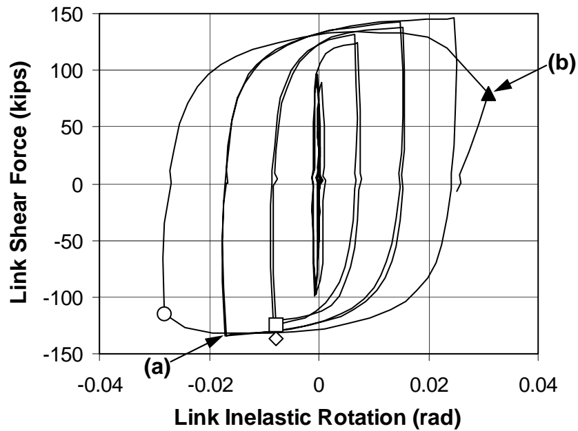
(b) Link Shear vs. Inelastic Rotation Angle
