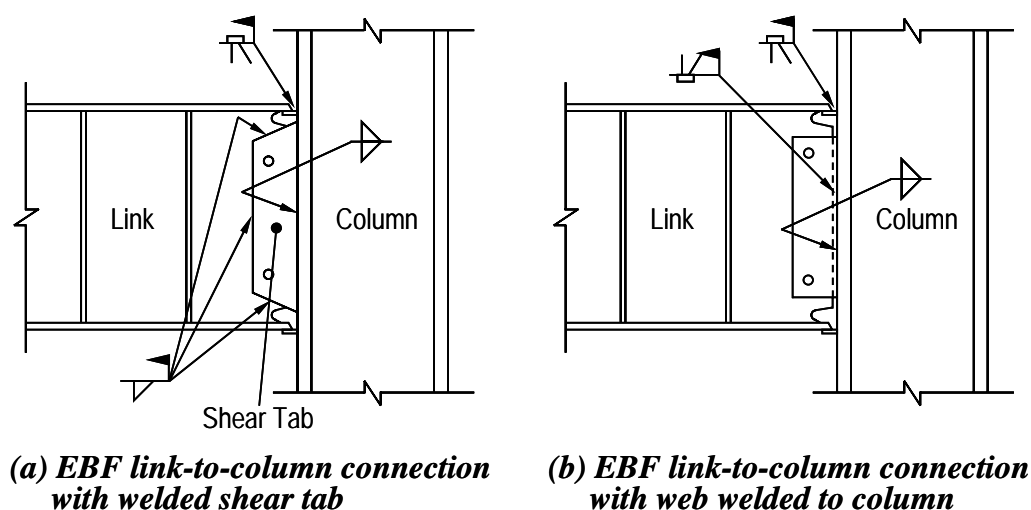
Figure 2.20 Pre-Northridge connections
