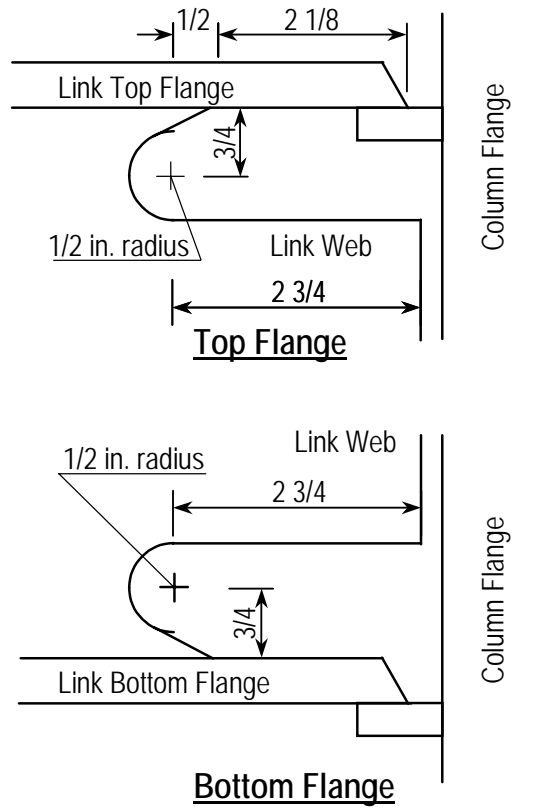
(c) FF-connections
