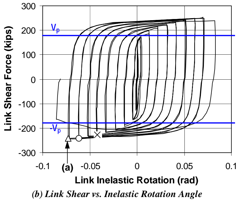
Figure 4.28 Response of Specimen NAS
