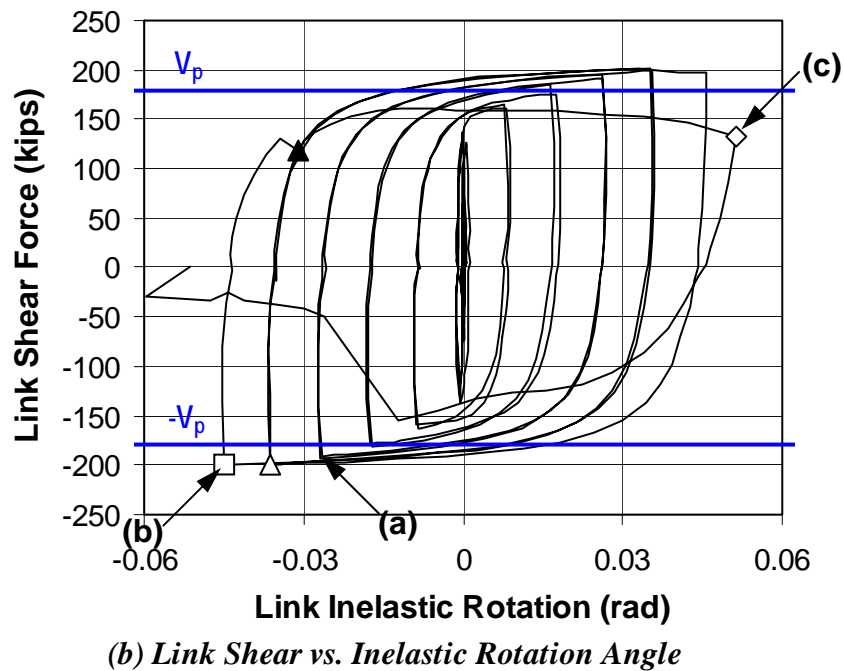
Figure 4.19 Response of Specimen FF1
