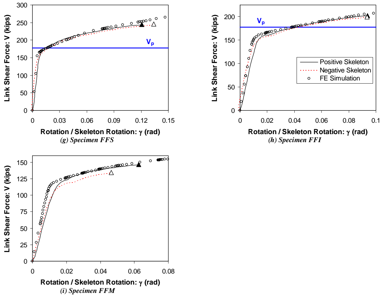
Figure 6.8 Simulated loading curve vs. skeleton curves (Continued)
