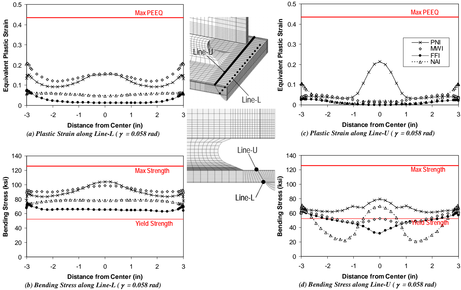
Figure 6.26 Link flange-groove weld interface in I-links
