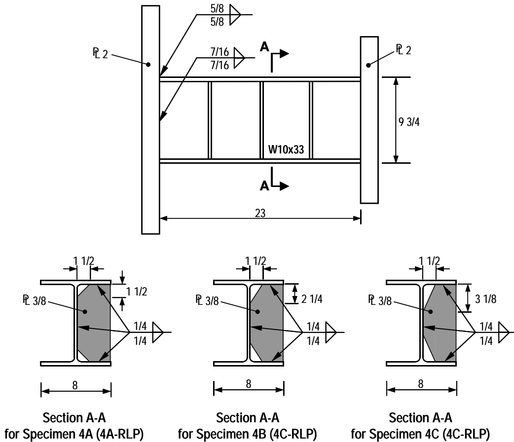
Figure 2.10 Termination of link stiffener welds in Specimens 4A, 4B, and 4C
