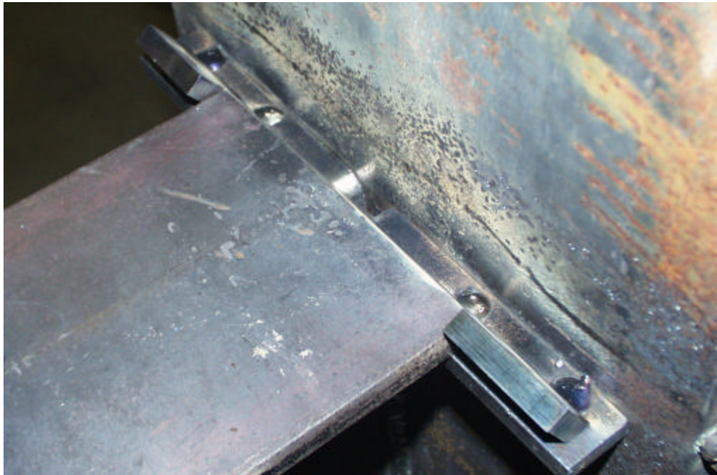
Figure E11 Tack welds for link top flange of Specimen NASL-RLP
