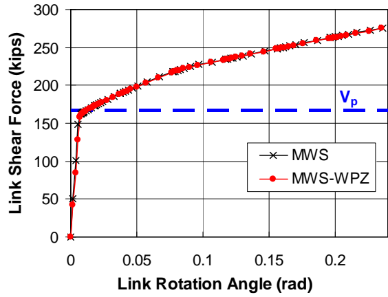
(a) Link Shear vs. Rotation Angle
