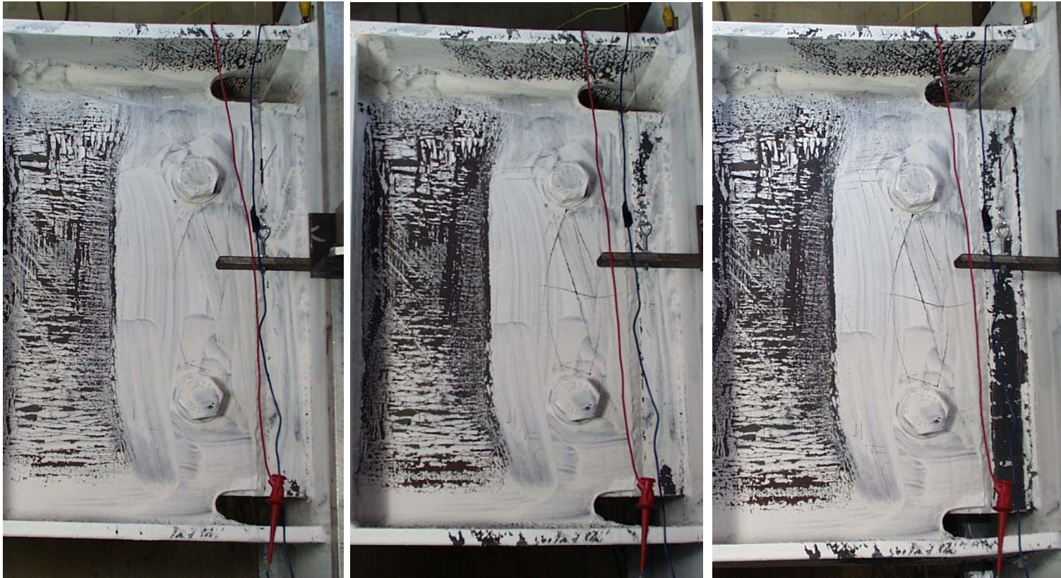
Figure 4.26 Photographs of Specimen FFSL-RLP:
