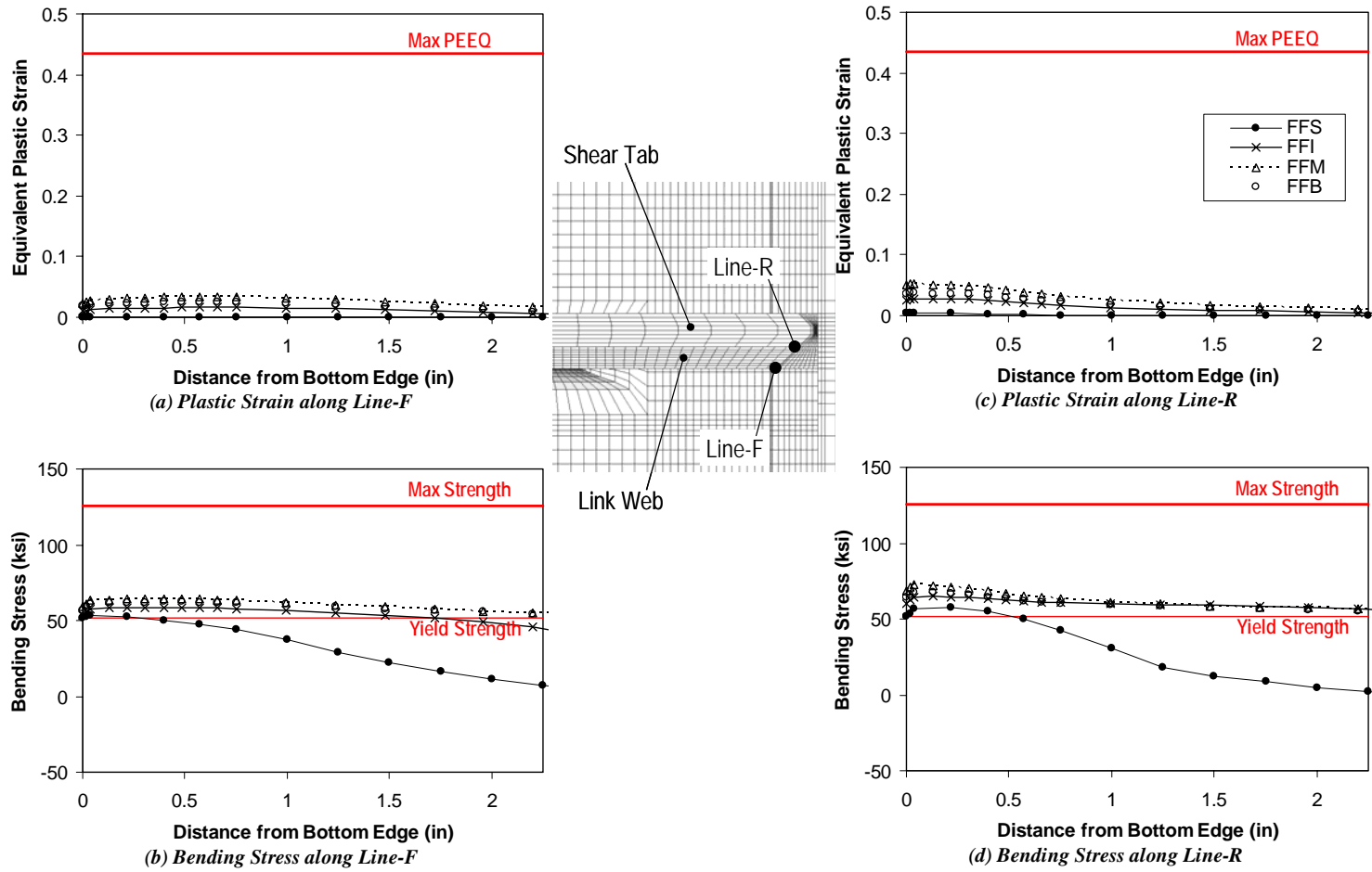
Figure 6.29 Link web-groove weld interface in FF-models
