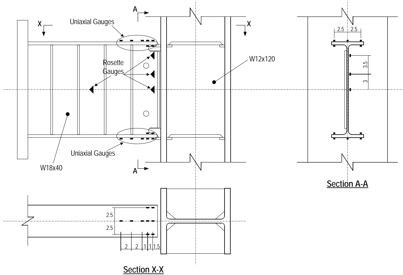
Figure 3.11 Strain gauge location for MWS
