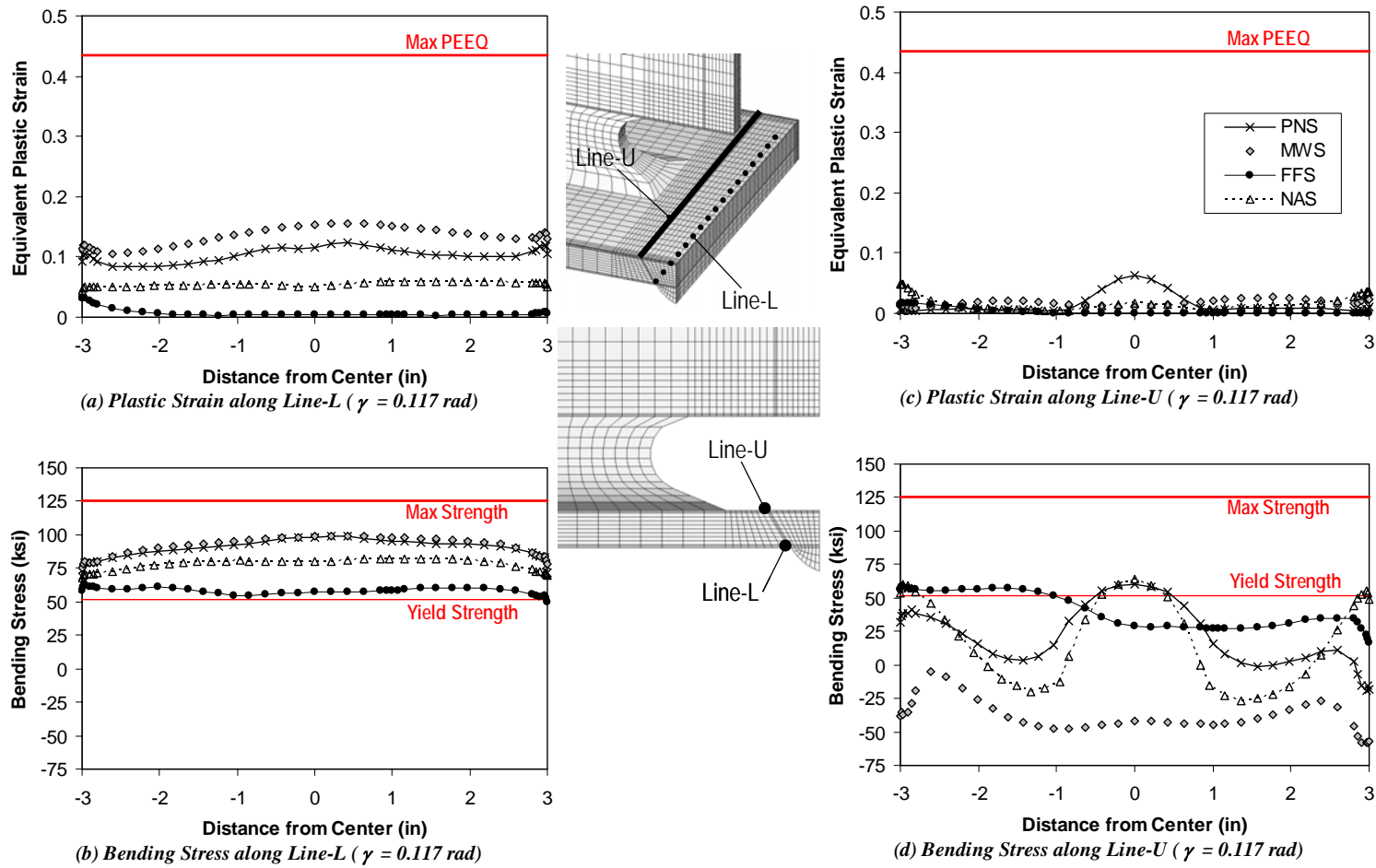
Figure 6.25 Link flange-groove weld interface in S-links
