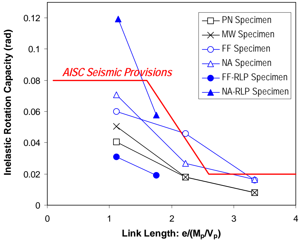
Figure 4.38 Link Rotation Capacity
