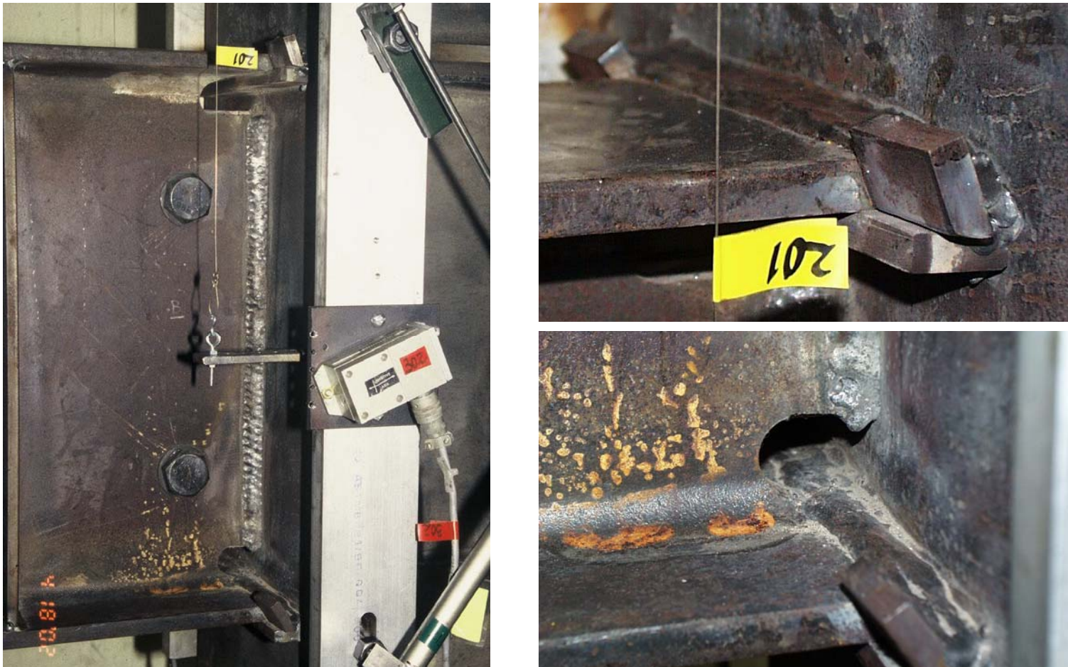
Figure 4.1 Specimen PNI: Connection before testing: (a) (Above) Entire view; (b) (Above right) Link top flange groove weld; (c) (Below right) Link bottom flange groove weld
