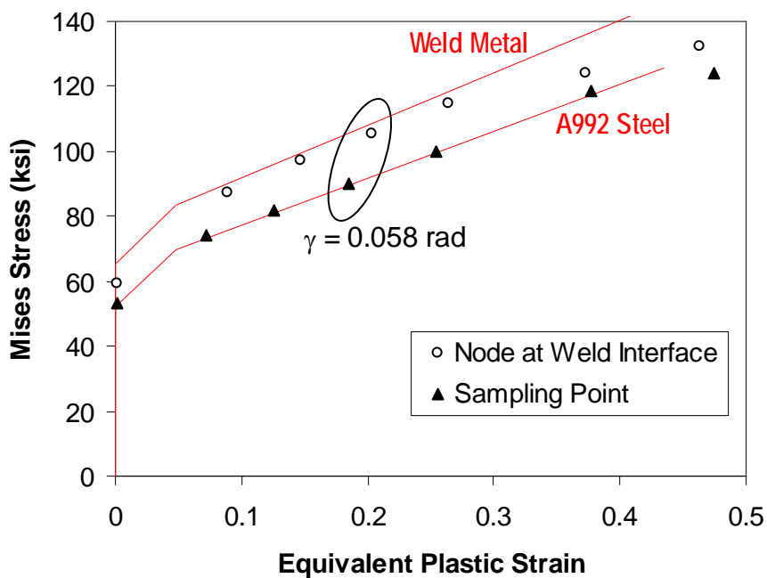
Figure 6.20 Stress-strain relationship measured at sampling point
