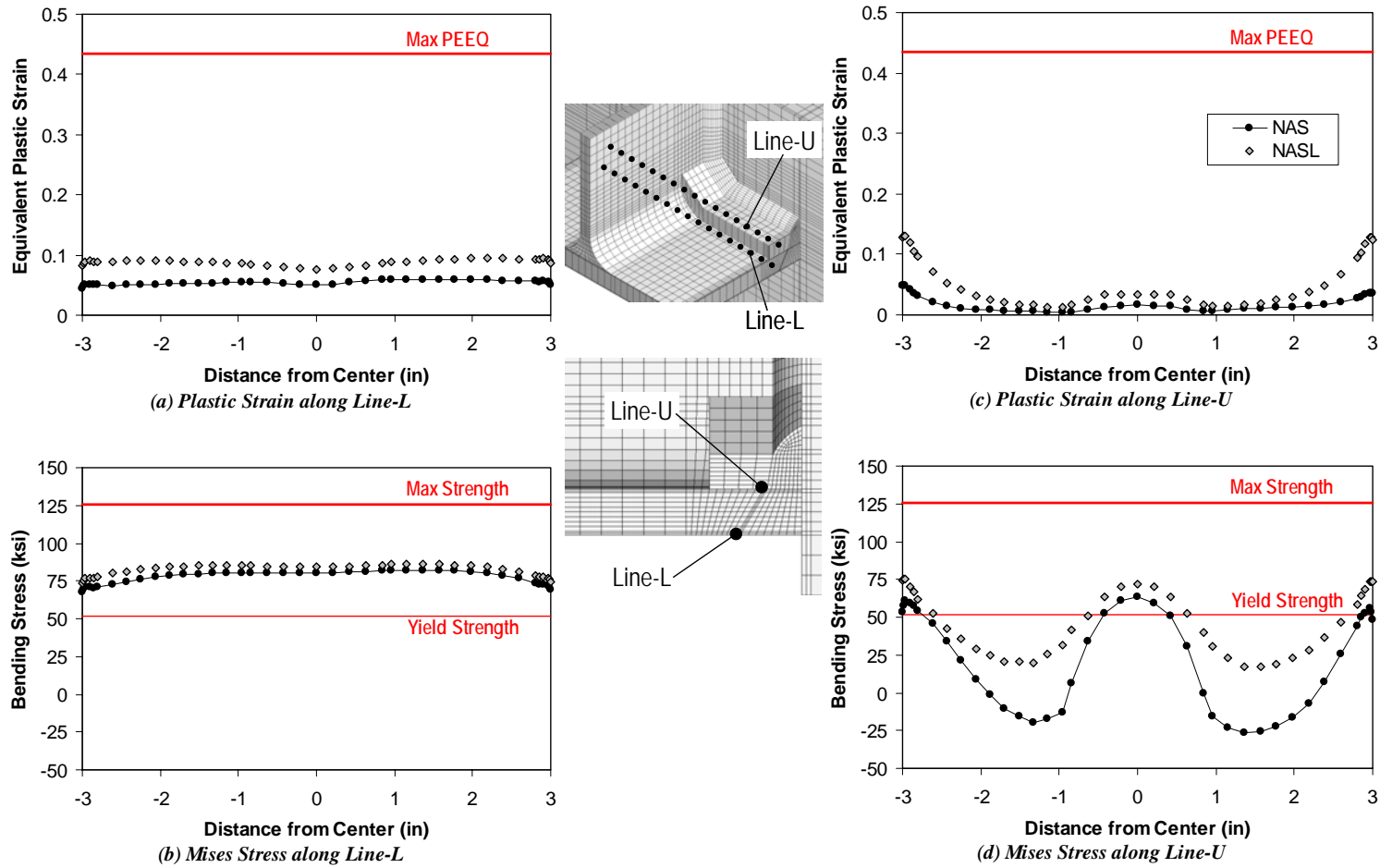
Figure 6.31 Comparison between Model NAS and Model NASL-RLP
