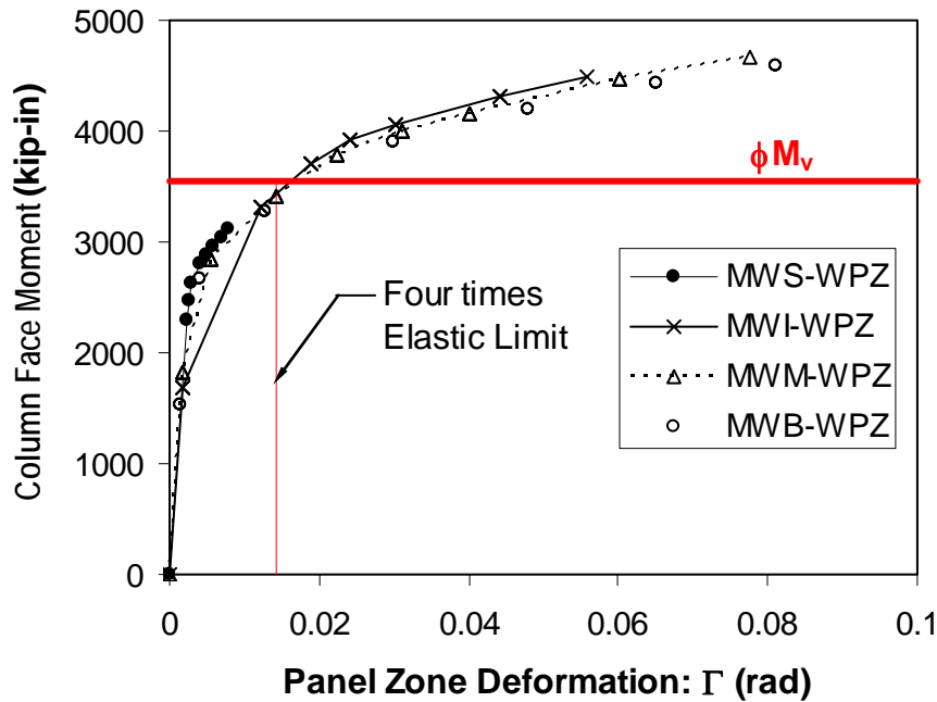
Figure 6.34 Column face moment vs. panel zone deformation
