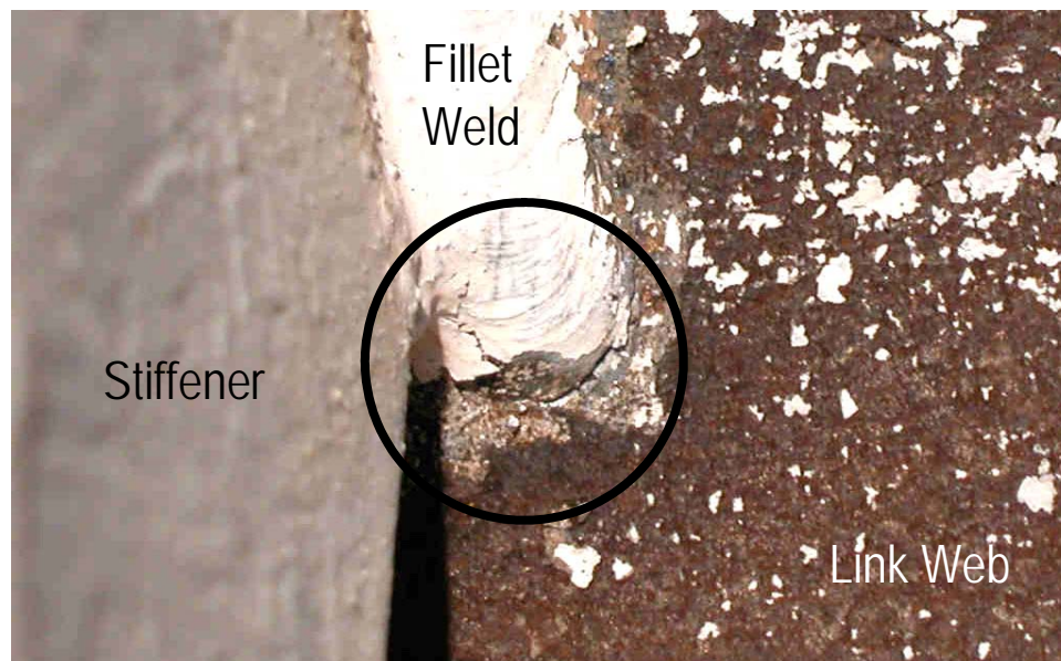
Figure 2.11 Fracture initiation in link web of Specimen 4A-RLP (Ryu et al. 2004)
