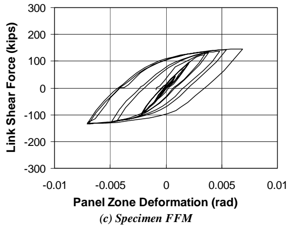
Figure 5.29 Panel zone deformation vs. link shear
