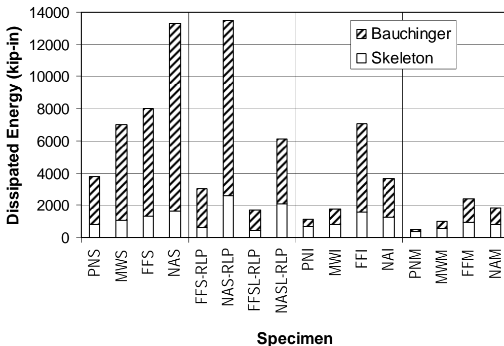
Figure 5.10 Skeleton energy and Bauschinger energy
