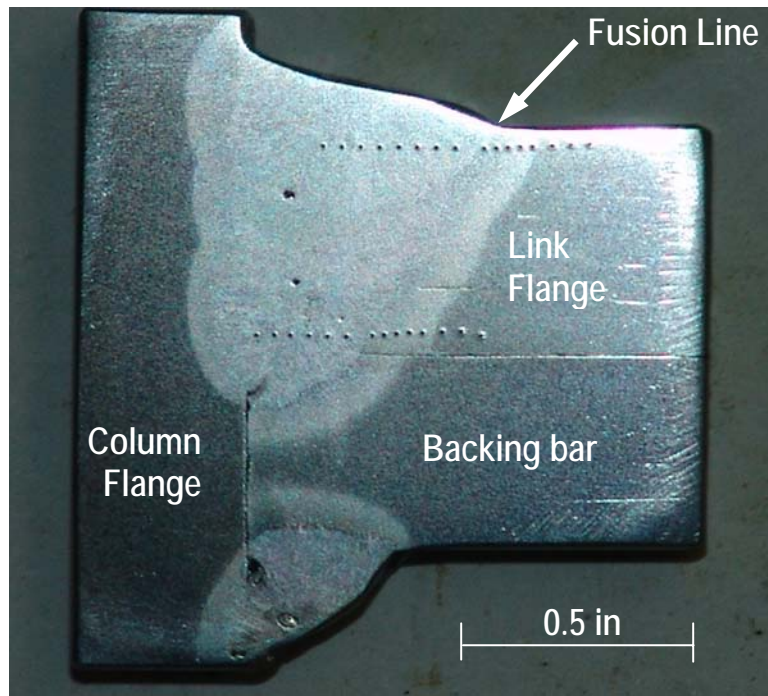
(a) Acid-etched E70T-6 weld
