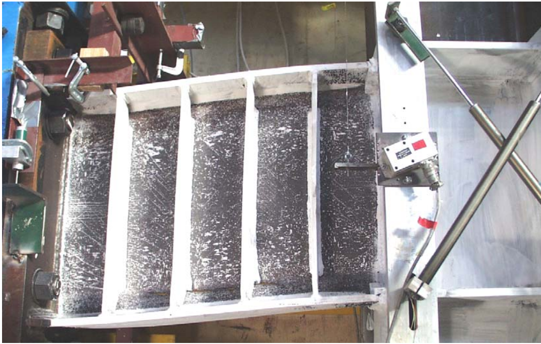
(a) Horizontal fracture in link web (0.09-1P)
