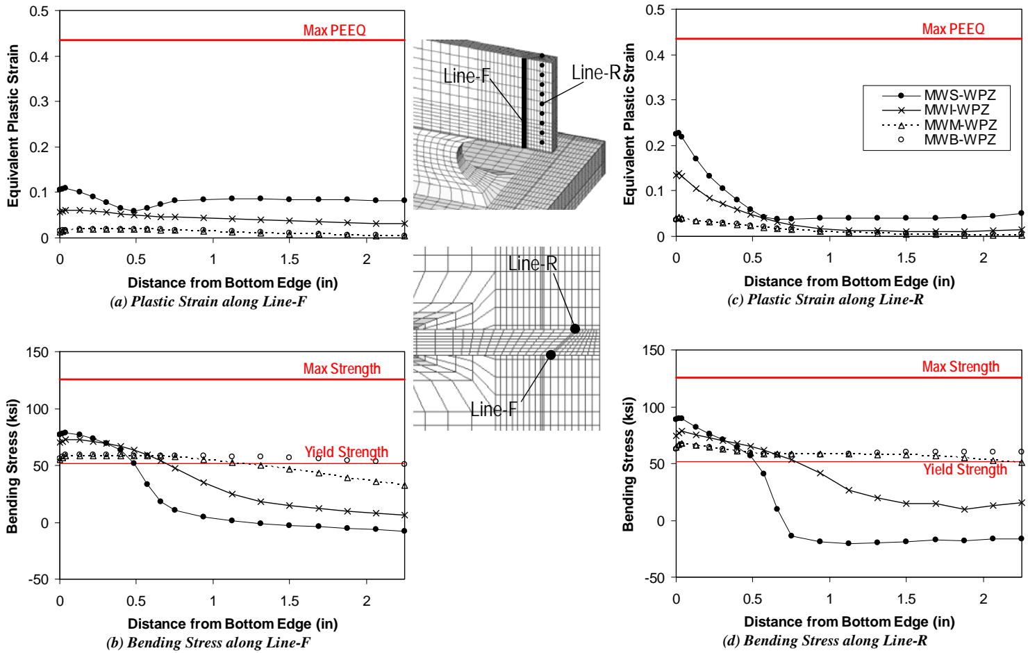
Figure 6.37 Effect of weak panel zone in link web weld interface
