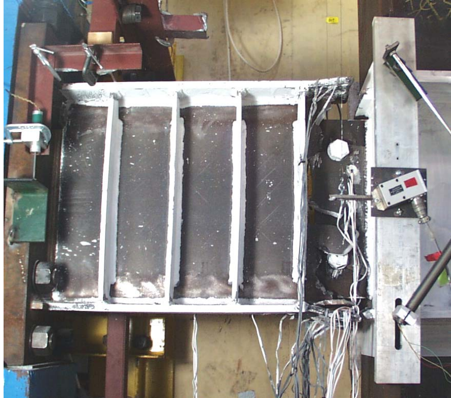
Figure 4.10 Photographs of Specimen MWS (Continued): (c) (Left) Link top flange separated from column face (0.07-2P); (d) (Above) Link after test
