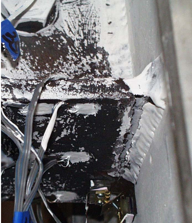
(a) Fracture in link bottom flange (0.03-1N)
