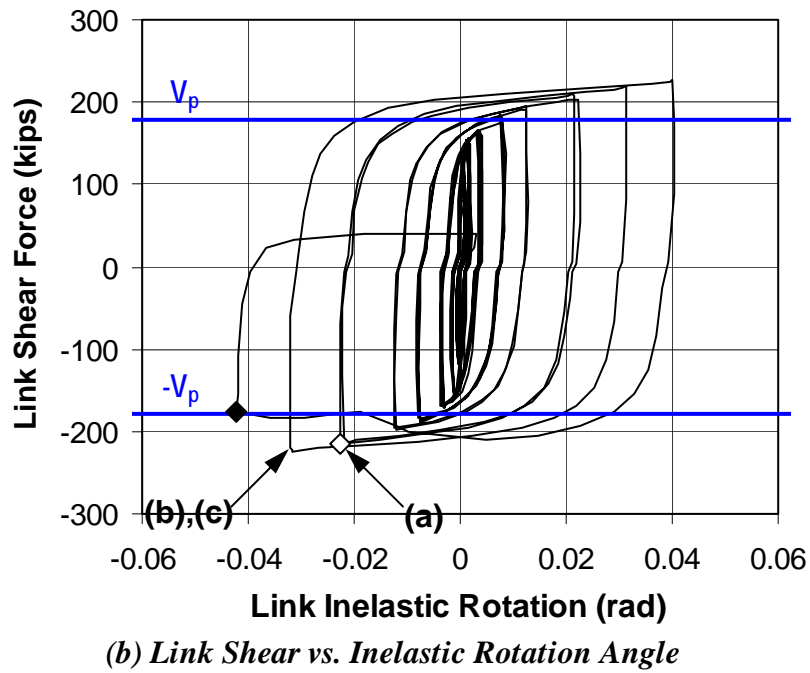
Figure 4.23 Response of Specimen FFS-RLP
