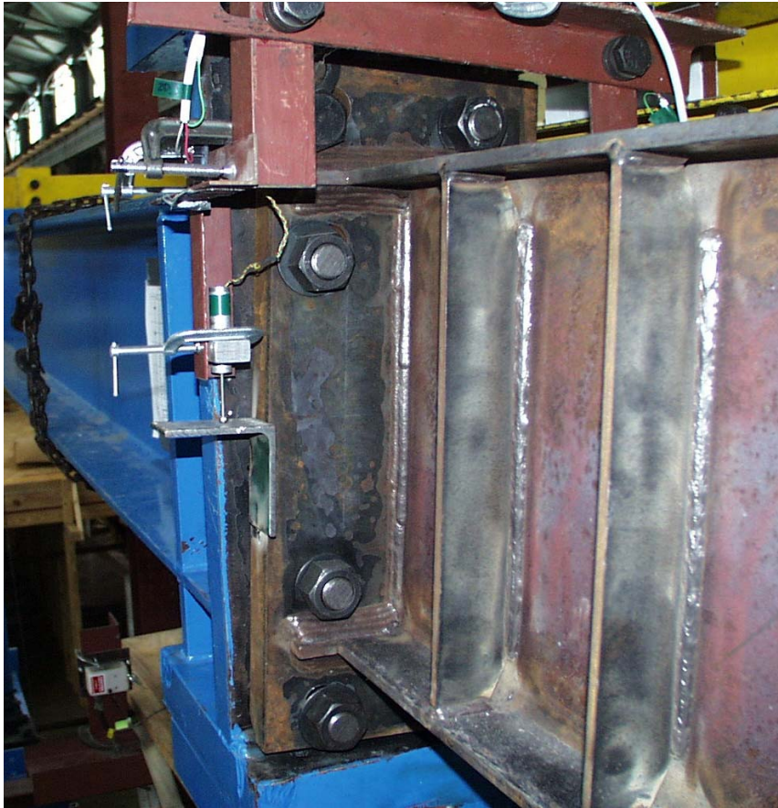
(a) Initial imperfection visible at beam end of link
