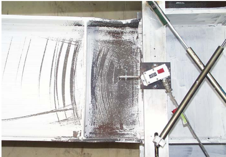
(b) Tested link and panel zone at \gamma = 0.04 rad
