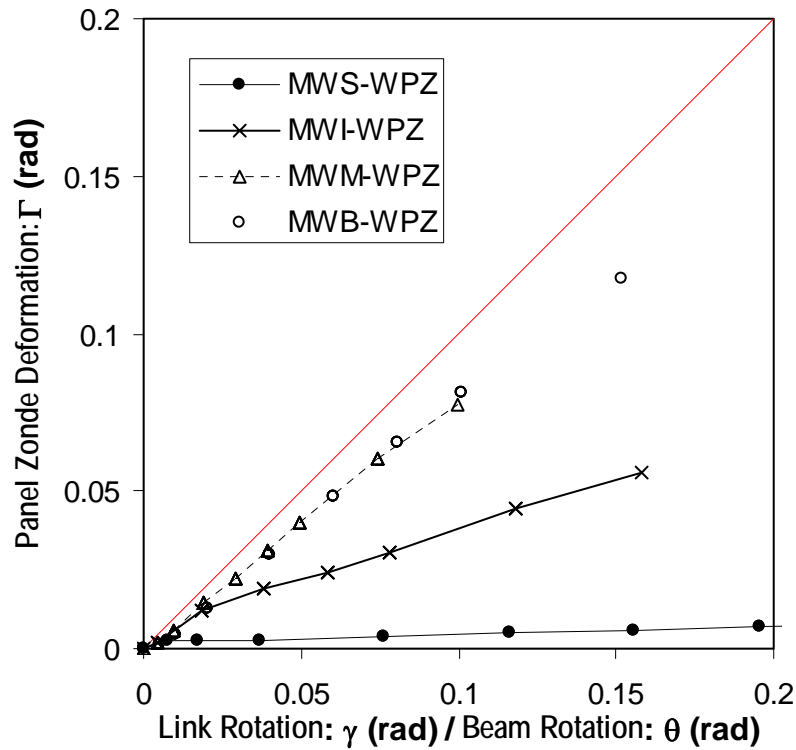
Figure 6.33 Contribution of panel zone deformation
