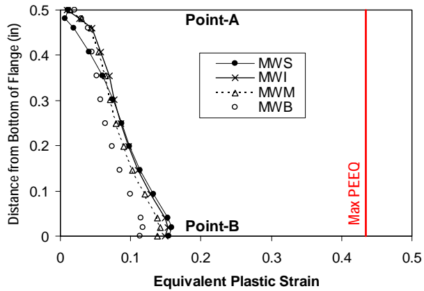
(a) Plastic Strain along Thickness of Flange
