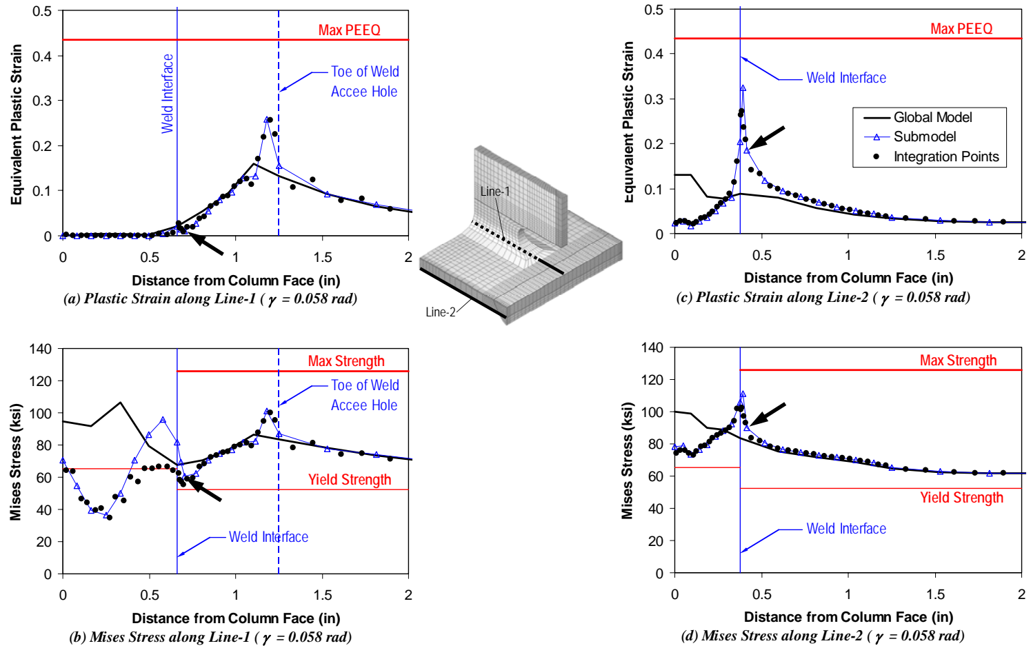
Figure 6.18 Sampling points near link flange groove weld
